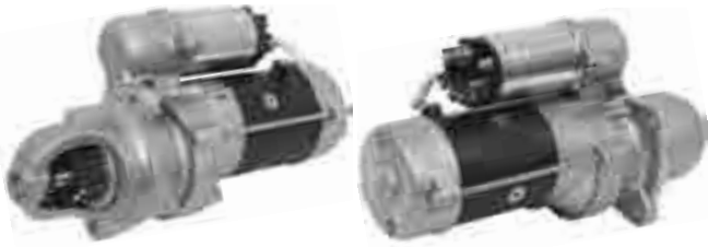
50-8441 (Ref# 79606N) Starter - Delco 28MT Series 12 Volt, CW, 12-Tooth Pinion
