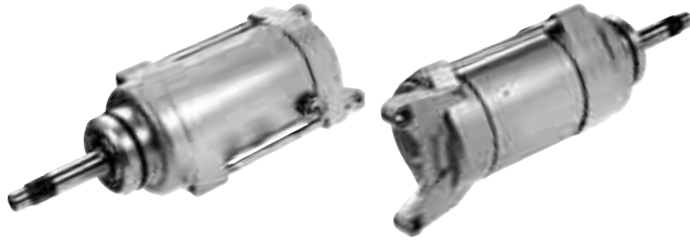
2-2176 (Ref# S8000N, ME3277-NA) Starter - Motorcycles 12 Volt, CW, 31-Spline Shaft
